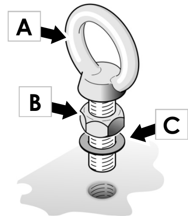
Figure 9. Installing an eyebolt
